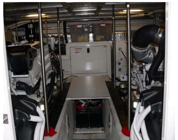
[below] Looking forward into engine room: Volvos each side, Kohler generator at forward end. Bow thruster batteries are under raised bilge floor forward.
